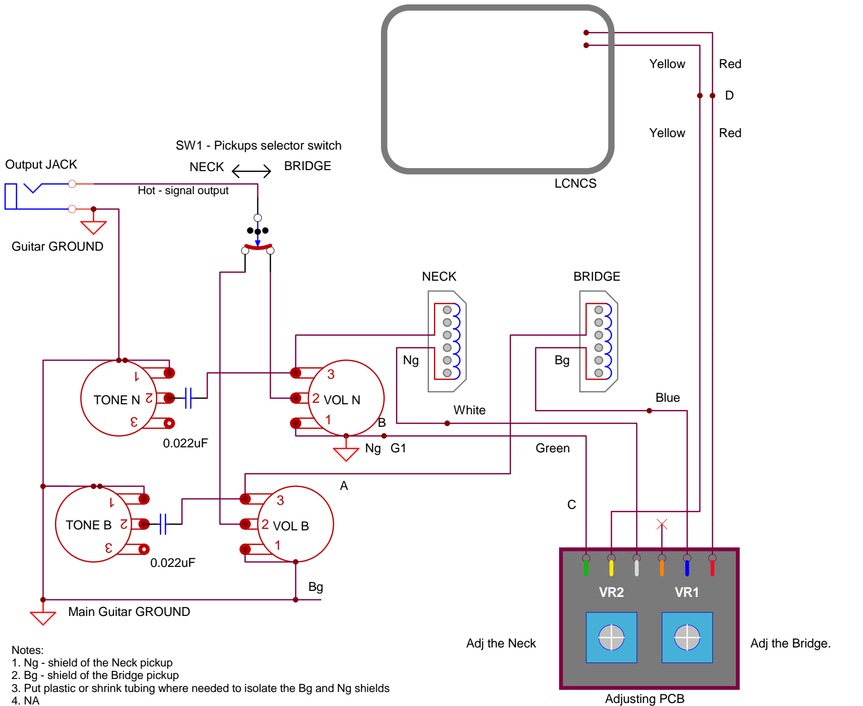
LCNCS Wiring diagram. Bridge and Neck pickups with braided wires All rights reserved, ILITCH ELECTRONICS LLC
